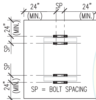
TYPICAL CONCRETE EDGE DETAIL
