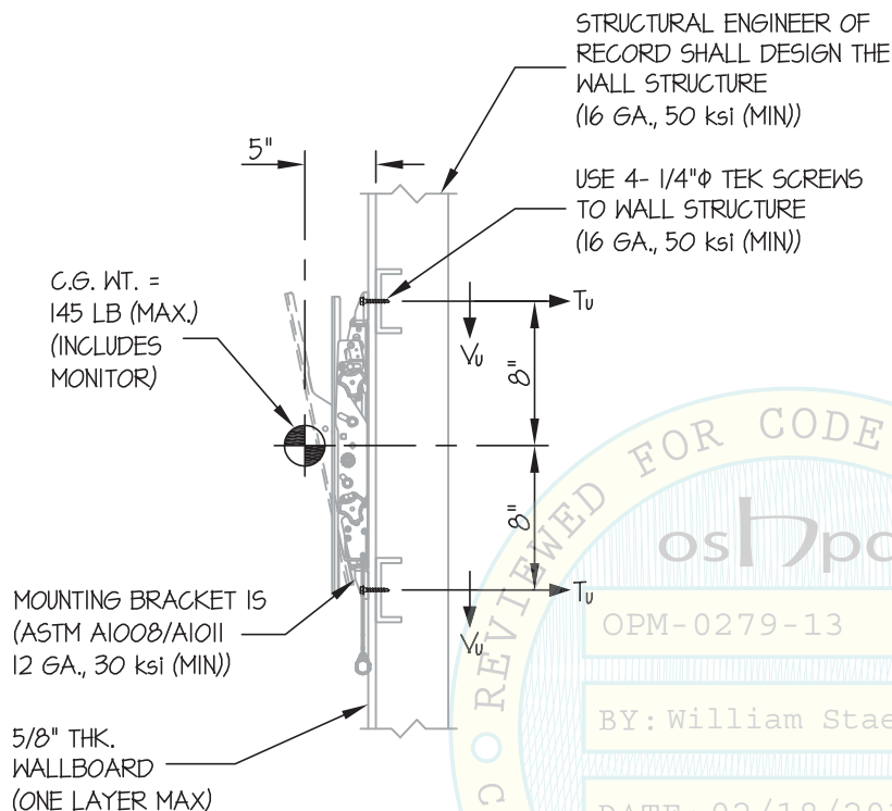
STEEL STUD WALL SECTION (MTMIU MODEL SHOWN)
