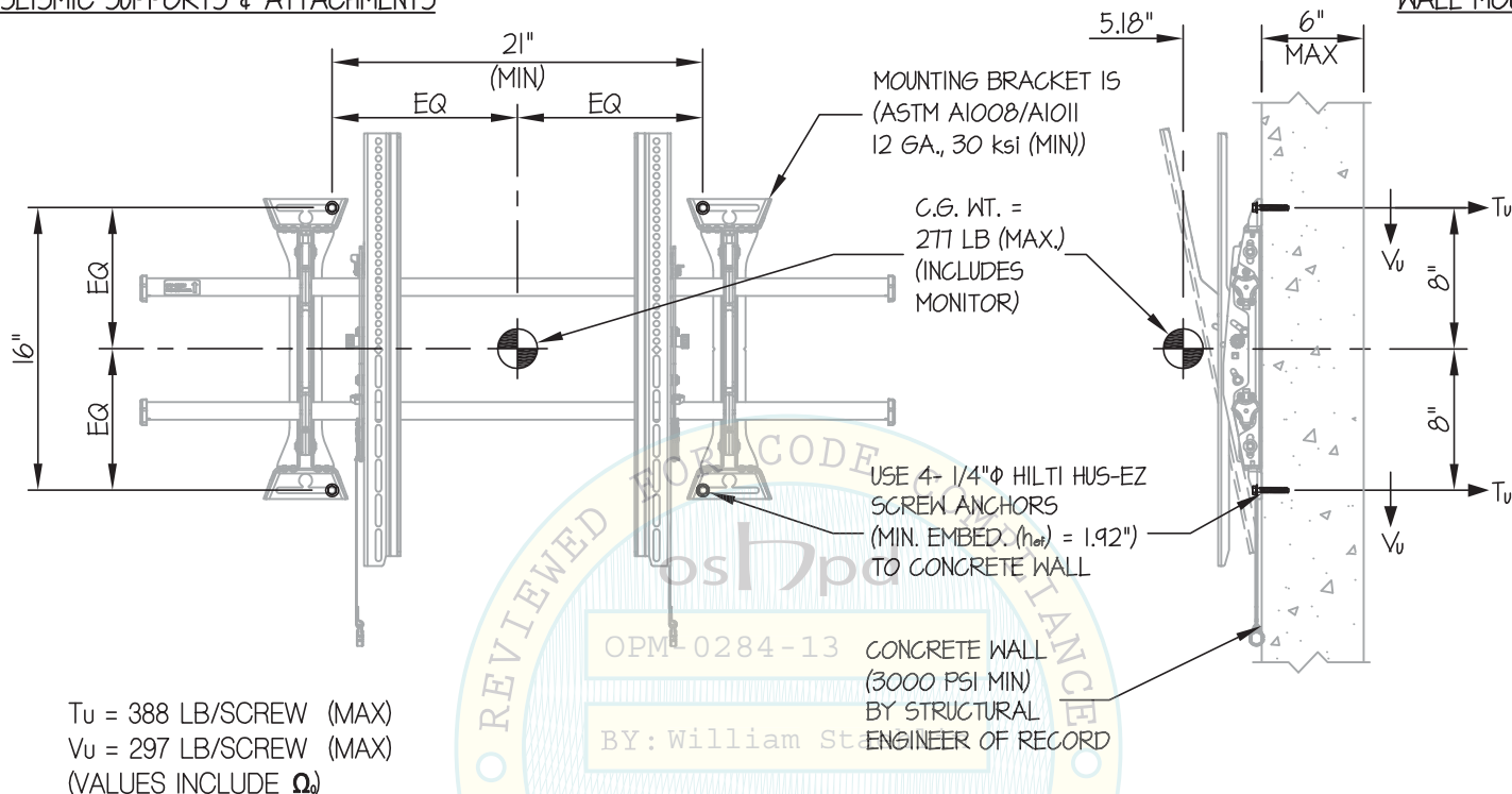
ELEVATION AT WALL PLATE (XTM1U MODEL SHOWN)
