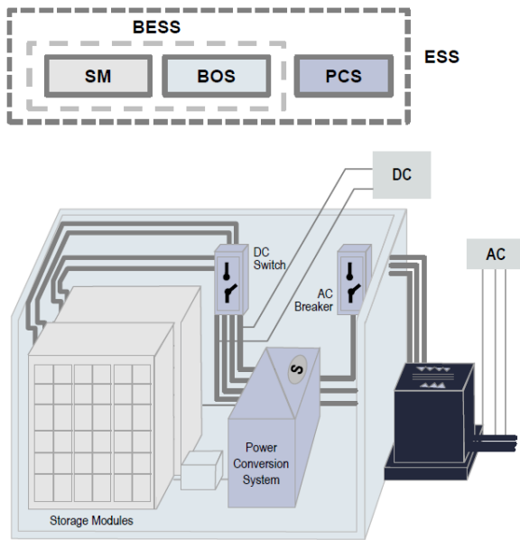
Figure 11: BESS Primary Elements (Lazard 2017).
